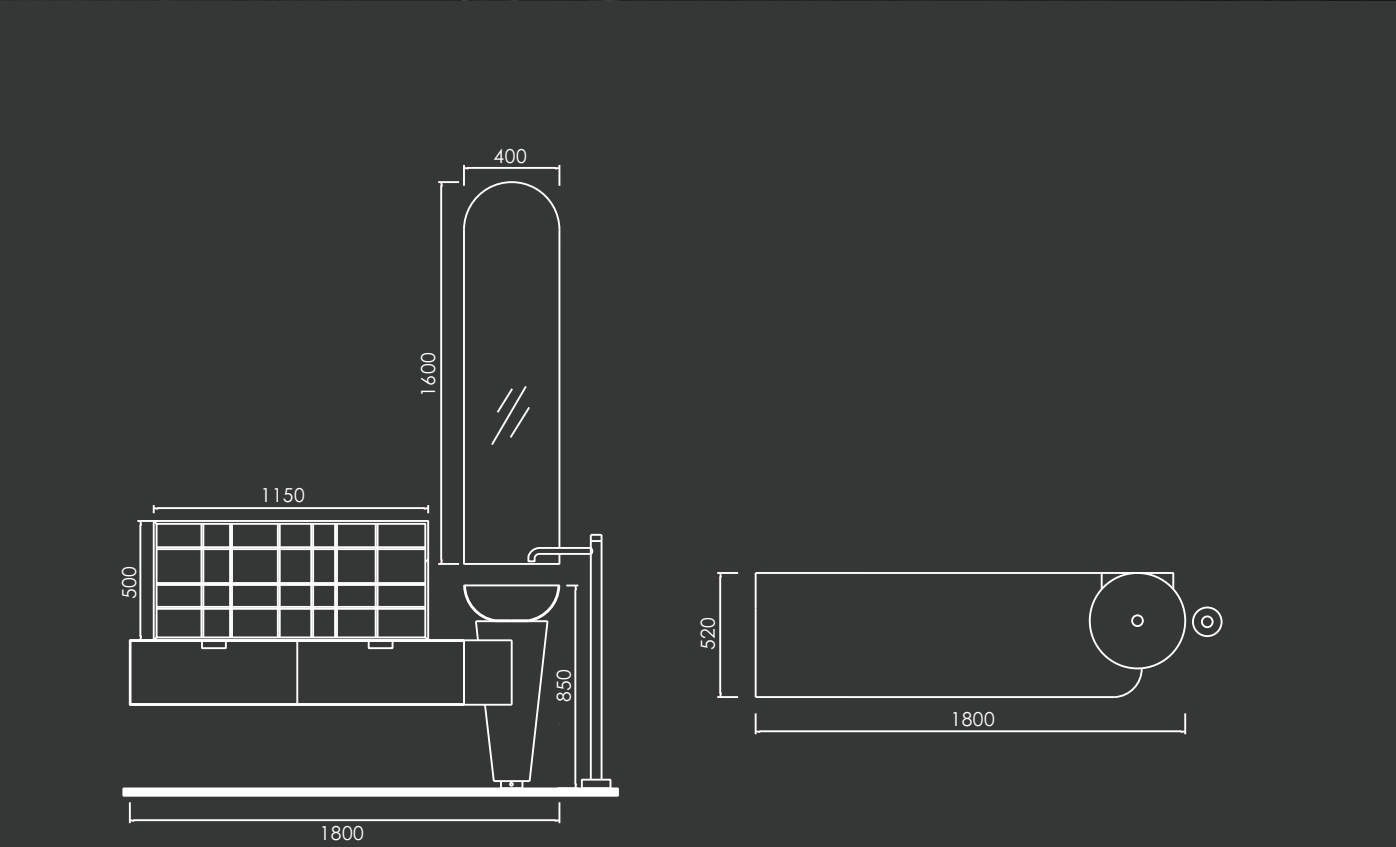
AL-22-3128 MAIN CABINET: 1800 x 520 x 850 mm MIRROR: 400 x 45 x 1600mm SHELF: 1150 x 150 x 500mm
